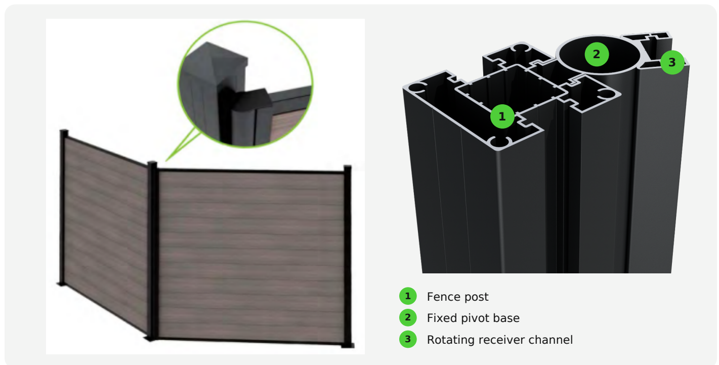
Angled fence application and installed swivel connection detail
